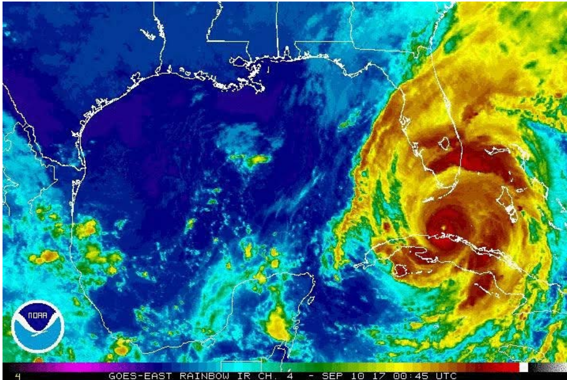
Hurricane Irma
